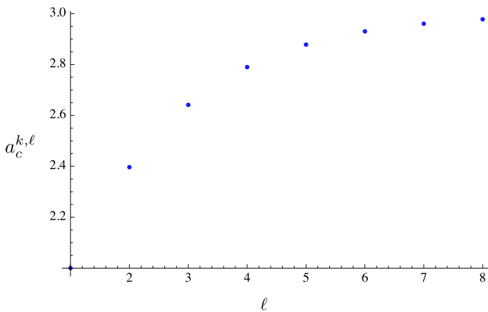
Fig. 4 A plot of a_c^{(k, \ell)} for k = 1 and \ell = 1, 2, 3, \dots, 8 . The point (1, 1) is Dyck paths, where a_c = 2 , and the limiting value a_c|_{k=1, \ell=\infty} = 3 is the Motzkin path bijection point. The latter bijection point has non-standard surface weights ( i.e. the bijection is not weight preserving) and hence a_c \neq 3/2
