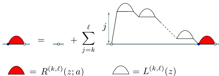
Fig. 3 Schematic representation of the Lukasiewicz path factorisations
