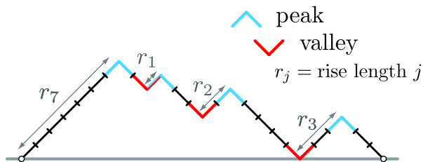
Fig. 6 An example of a Dyck path shown the rises, hook, peaks and valleys
