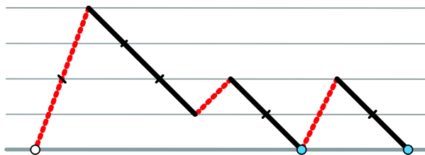
Fig. 2 An example of a (1, 2)-restricted Lukasiewicz path of length eleven with two contacts. The jump steps are shown in colour (dashed)
