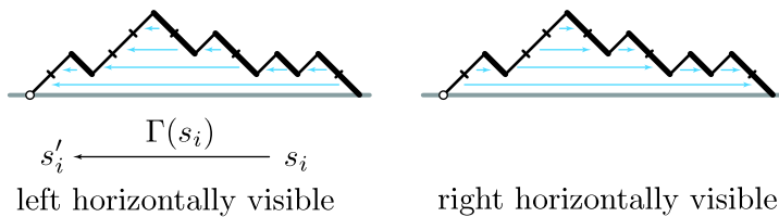
Fig. 7 Horizontally visible steps—to the left ( left ) or to the right ( right )
