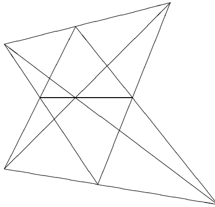
Figure 3: Pappus' Theorem
