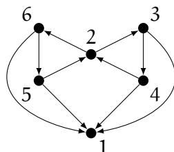
Figure 6.4: Output gadget, used in the proof of Theorem 6.11. All players have payoffs as in Figure 6.3. Player x must play action 0 in every pure equilibrium of the game.
