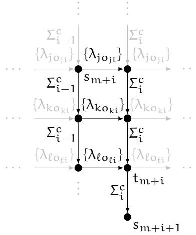
Figure 5.11: Gadget for clause c_i = (x_j \vee x_k \vee x_\ell) used in the proof of Theorem 5.22. o_{ji} denotes the number of times variable x_j occurs in clauses up to and including c_i .
