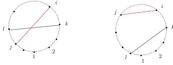
Figure 4: The left pair is admissible while the right pair is not admissible
