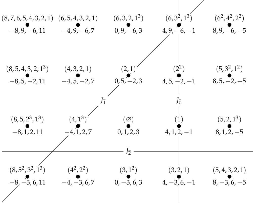
Figure 4: 5-cores inside the lattice of self-conjugate 4-cores
